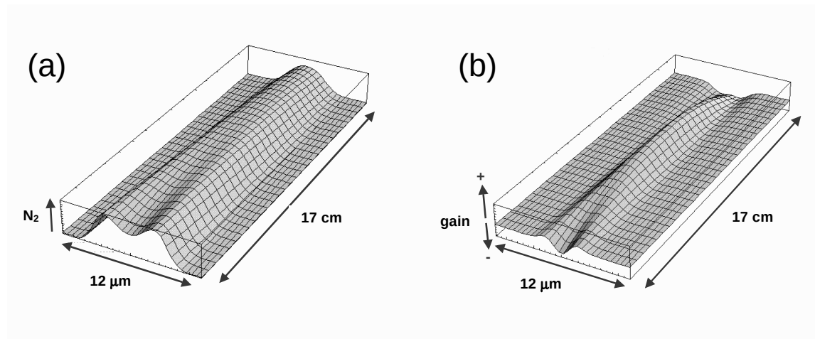
Figure 2.3. (a) Fraction of Er in the first excited state along a 2\ \mu\text{m} wide, 17 cm long ridge waveguide, calculated in the plane of the waveguide. The waveguide is pumped with 100 mW at 1.48\ \mu\text{m} . The maximum fraction of excited Er that is reached is 68%. The dip near the front facet is caused by excited state absorption. (b) Differential gain calculated from the excited Er distribution and the optical mode of the signal.
