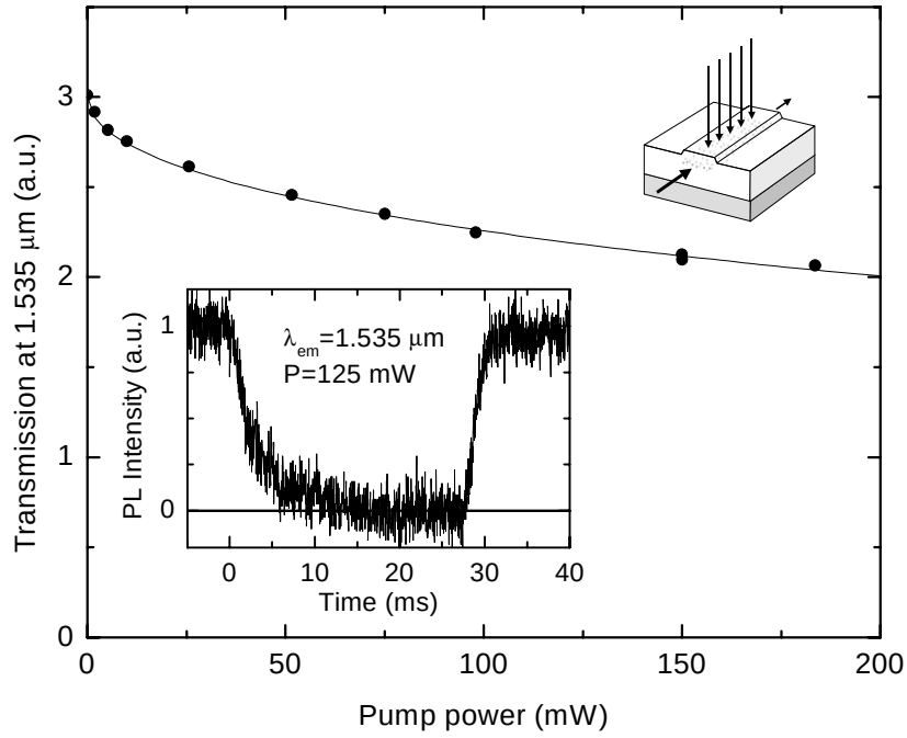
Figure 9.3. Waveguide transmission at 1.535 \mu m as a function of the applied continuous-wave 458 nm pump power. A sketch of the measurement configuration is included. The inset shows the time-dependent photoluminescence signal at 1.535 \mu m collected at the output facet during pump modulation.
