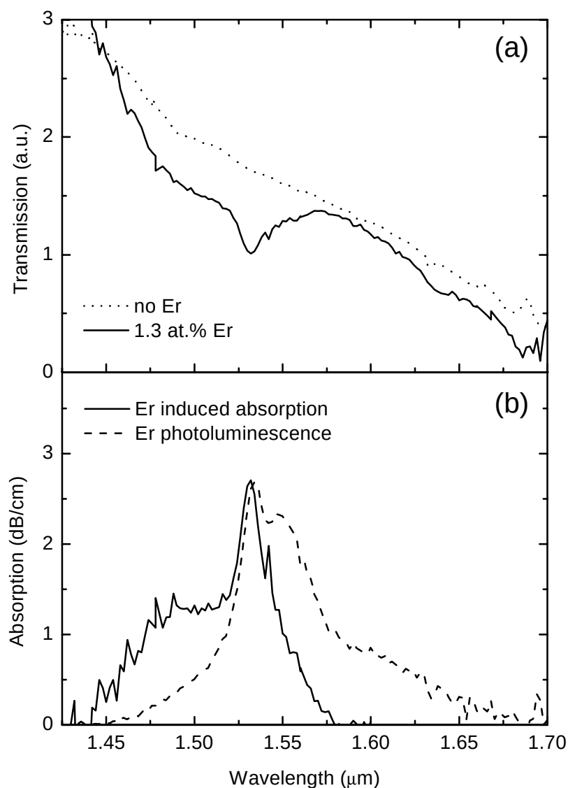
Figure 9.2. (a) Normalized transmission spectra of Si nanocrystal based waveguides containing no Er (dotted line) and 1.3 at.% Er (solid line) (b) Er related absorption spectrum (solid line) derived from the data in (a) and Er photoluminescence spectrum (dashed line) collected at the waveguide output facet (pump power 180 mW at 458 nm).
