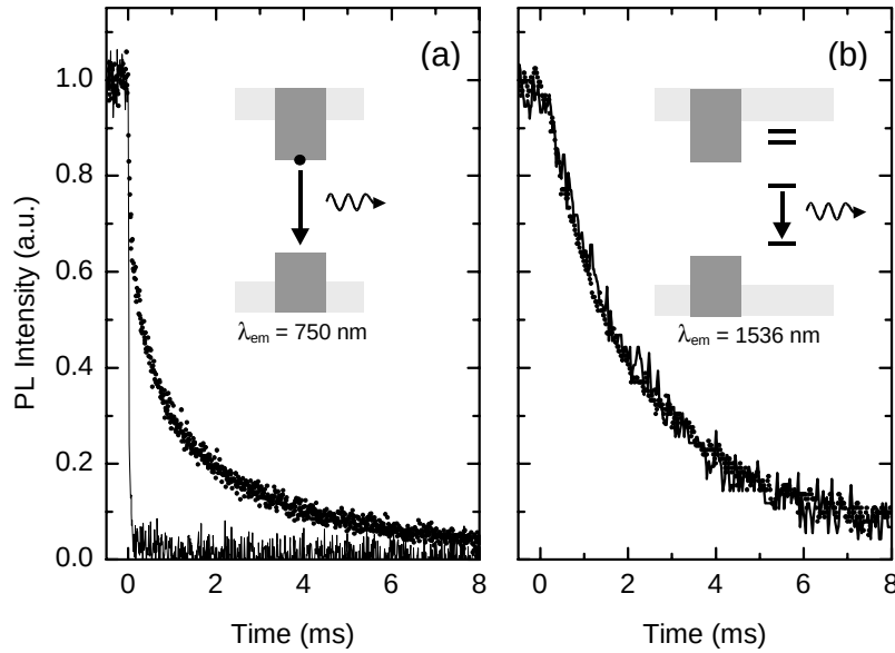
Figure 7.4. Luminescence decay measurements taken at 15 K (dots) and at 300 K (drawn lines) of (a) nanocrystal luminescence at 750 nm, and (b) Er^{3+} luminescence at 1536 nm.
